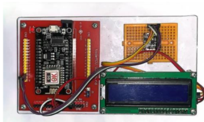
Picture 1. Prototipe Starter IoT Oxymeter
