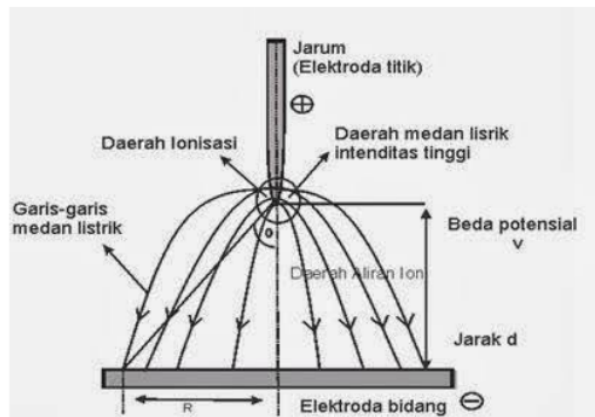
Figure 1.3 Plasma Formation Process
