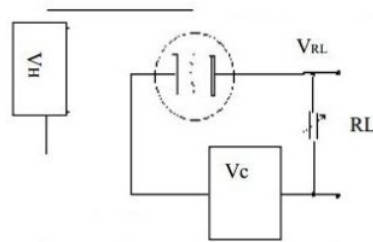
Figure 1.5 MQ-7 Gas Sensor Circuit
