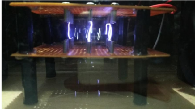
Figure 1.13 Corona Shape During the Filtration Process with Plasma Technology
