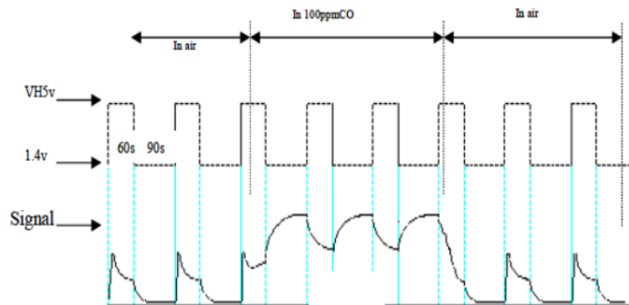
Figure 1.6 Principle of Operation of the MQ-7 Sensor
