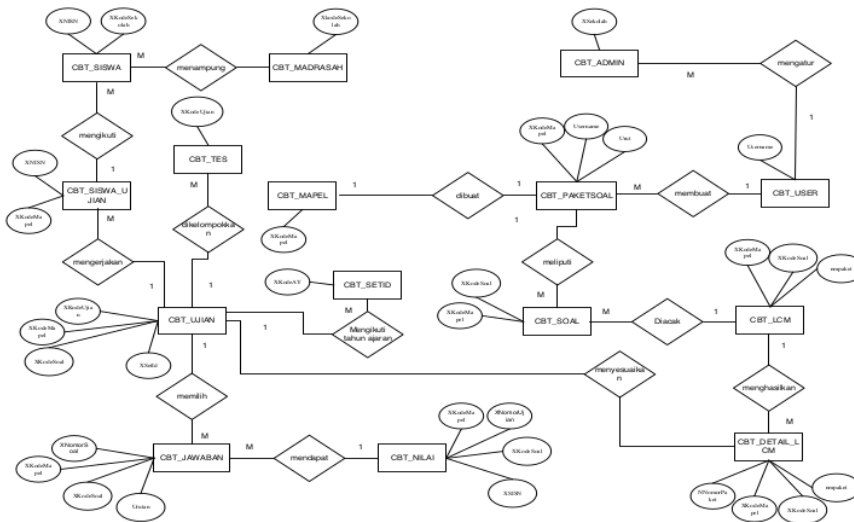
Figure 7 ERD
