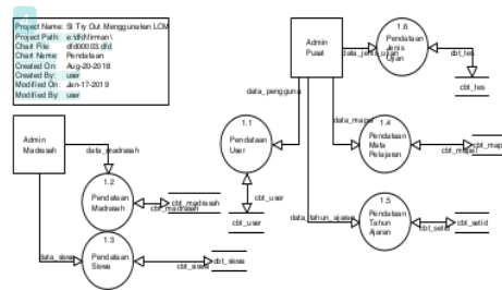
Figure 5 DFD Level 1 Data Collection
