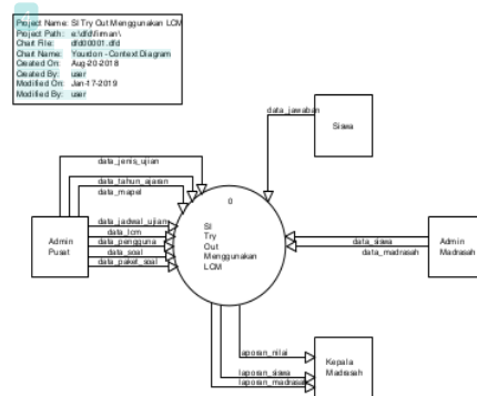
Figure 3 Context Diagram
