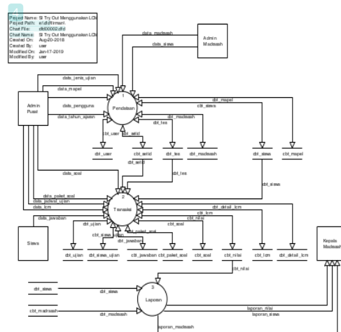
Figure 4 DFD Level 0
