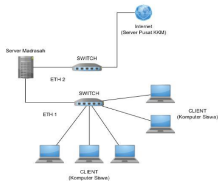
Figure 8 System Architecture
