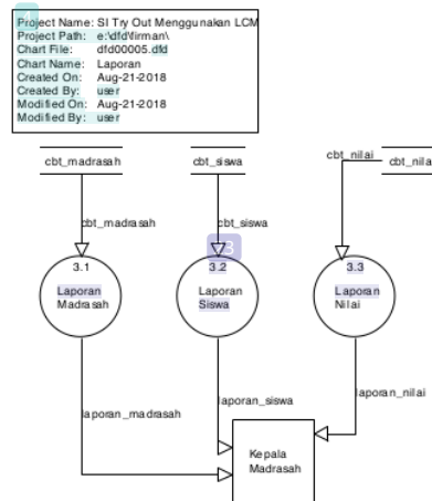
Figure 6 DFD Level 1 Report
