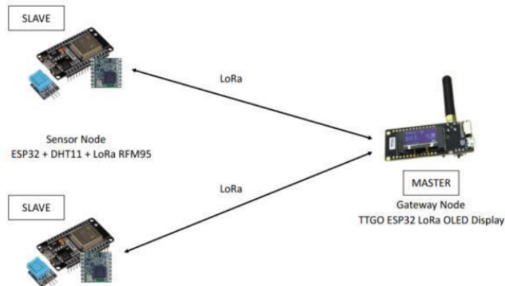
Figure 2. General Overview of System Architecture
