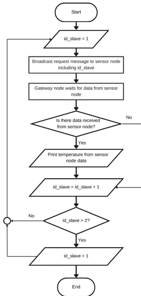
Figure 7. Flowchart Gateway node
