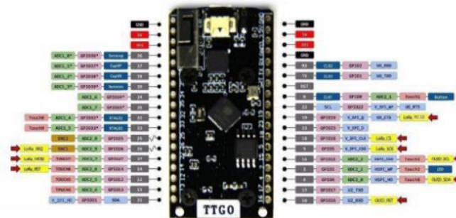
Figure 6. Pinout TTGO ESP32 LoRa OLED
