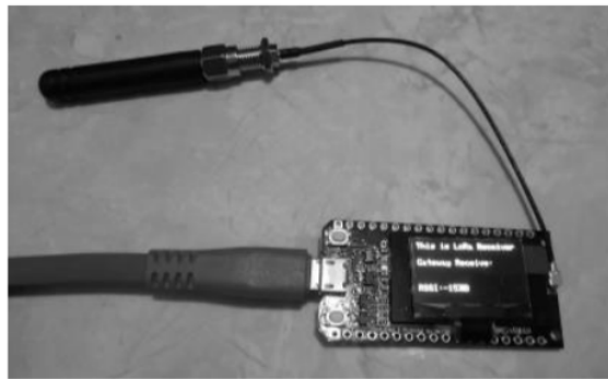
Figure 8. Microcontroller Gateway node
