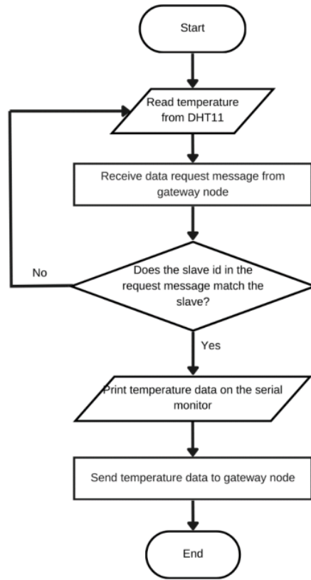
Figure 5. Flowchart of Sensor Node Design Workflow
