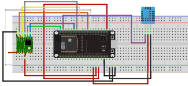
Figure 4. Sensor Node Architecture
