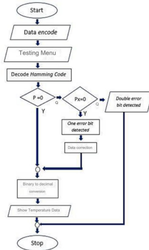
Figure 3. Decoding Flowchart for the Receiver
