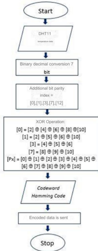
Figure 2. Hamming Code Encoding Flowchart for the Transmitter
