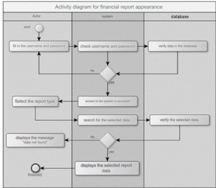
Figure 4. Activity Report Display Chart
