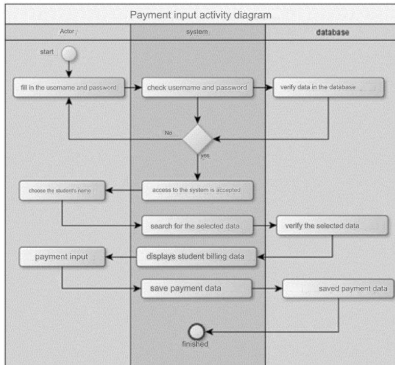
Figure 3. Payment Input Activity Chart
