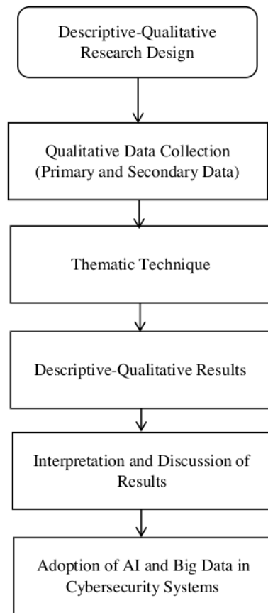
Figure 1: Research Framework
